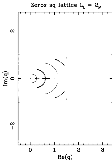
Fig. 5. Partition-function zeros in the complex q plane for the 2_p \times 20_F square-lattice strip for several values of the temperature-like parameter v : -1 ( \square ), -0.75 ( \circ ), -0.50 ( \triangle ), -0.25 ( \diamond ), and -0.10 ( \oplus ). The loci \mathcal{B} for the 2_p \times \infty_F strip for these values of v are also shown.
