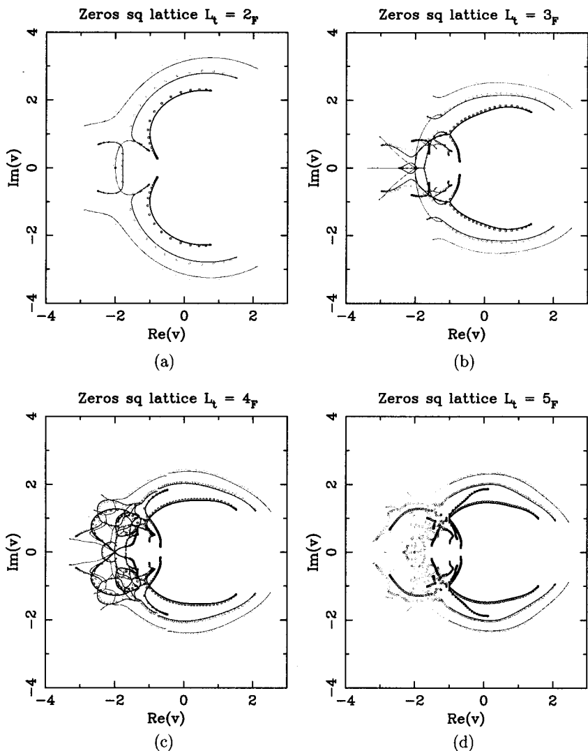
Fig. 9. Partition function zeros in the complex v plane for several square-lattice strips: (a) 2_F \times 20_F , (b) 3_F \times 30_F , (c) 4_F \times 40_F , and (d) 5_F \times 50_F . In each plot we show the zeros for several values of the parameter q : 2 ( \square , black), 3 ( \circ , red), and 4 ( \triangle , green) and the corresponding loci \mathcal{B} for these values of q . (Colors refer to the version of the paper online at cond-mat/0108144 at xxx.lanl.gov .)
