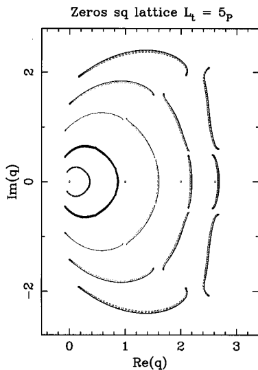
Fig. 8. Partition-function zeros in the complex q plane for the 5_p \times 40_F square-lattice strip for several values of the temperature-like parameter v : -1 ( \square ), -0.75 ( \circ ), -0.50 ( \triangle ), -0.25 ( \diamond ), and -0.10 ( \oplus ). The loci \mathcal{B} for the 5_p \times \infty_F strip for these values of v are also shown.
