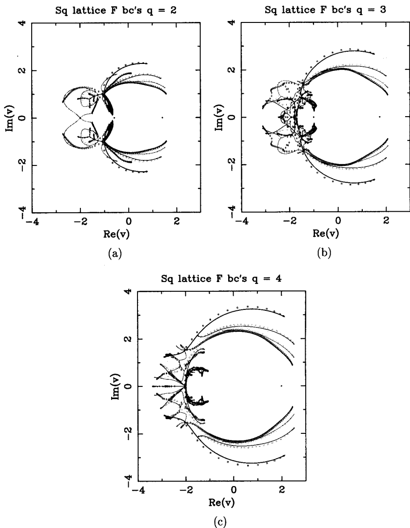
Fig. 11. Limiting curves forming the singular locus \mathcal{B} , in the v plane, for the free energy of the q = 2 (a) q = 3 (b), and q = 4 (c) Potts model on the (L_t)_F \times \infty_F square-lattice strips with the following widths L_t : 2 (black), 3 (red), 4 (green), and 5 (blue). We also show the partition-function zeros for the strips (L_t)_F \times (10L_t)_F for the same values of L_t : 2 ( \square , black), 3 ( \circ , red), 4 ( \triangle , green), and 5 ( \diamond , blue). (Colors refer to the version of the paper online at condmat/0108144.)
