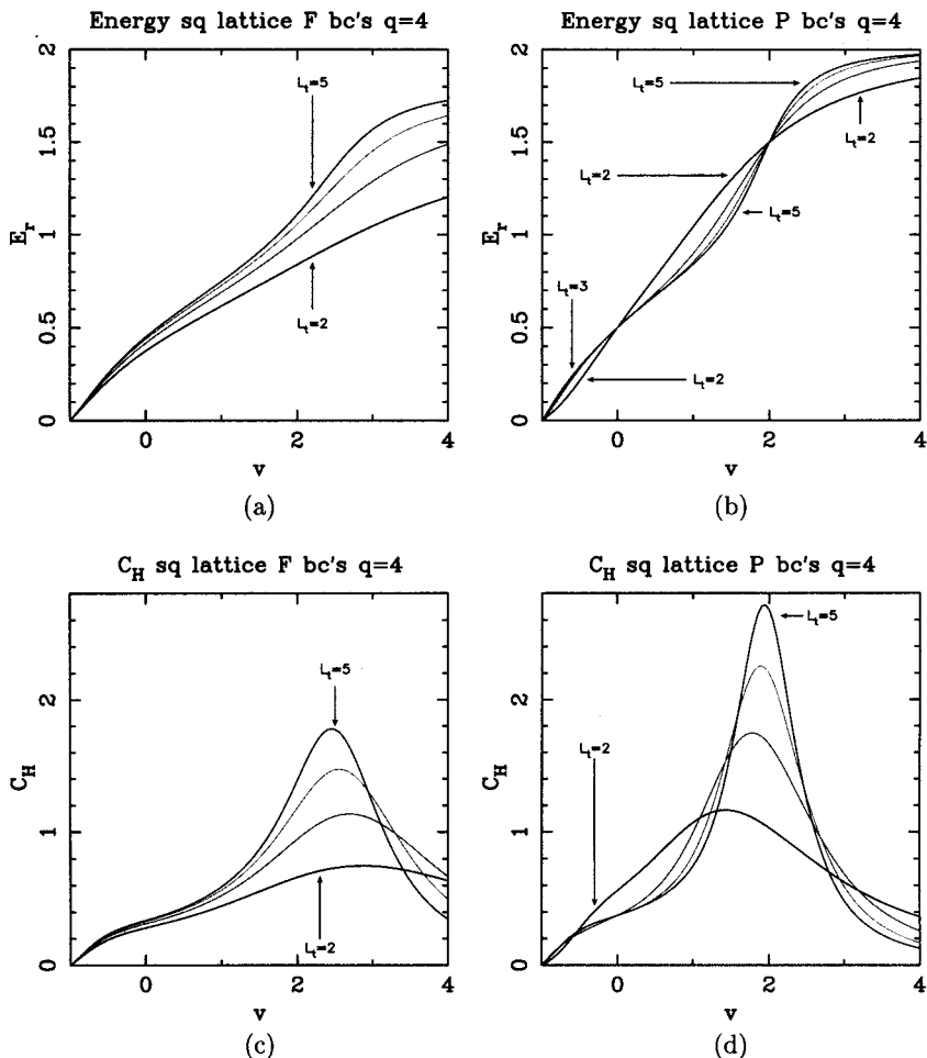
Fig. 15. Reduced internal energy E_r = -E/J and specific heat C_H as functions of v for the q=4 Potts model on square-lattice strips of size (L_t)_F \times \infty_F and (L_t)_P \times \infty_F with 2 \leq L_t \leq 5 . Notation is as in Fig. 13.
