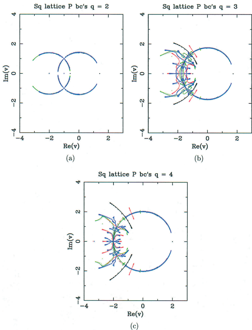
Fig. 12. Limiting curves forming the singular locus \mathcal{B} , in the v plane, for the free energy of the q=2 (a) q=3 (b), and q=4 (c) Potts model on the (L_t)_P \times \infty_F square-lattice strips with the following widths L_t : 2 (black), 3 (red), 4 (green), and 5 (blue). We also show the partition-function zeros for the strips (L_t)_P \times (10L_t)_F for the same values of L_t .
