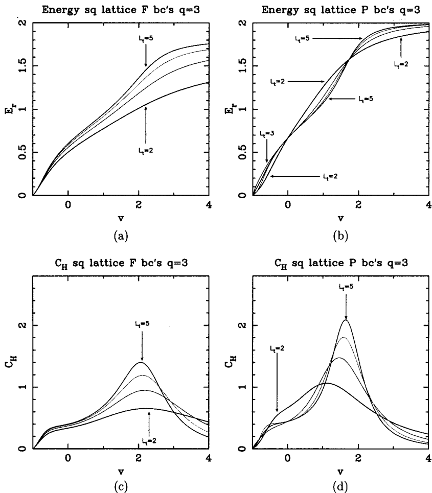
Fig. 14. Reduced internal energy E_r = -E/J and specific heat C_H as functions of v for the q=3 Potts model on square-lattice strips of size (L_t)_F \times \infty_F and (L_t)_P \times \infty_P with 2 \leq L_t \leq 5 . Notation is as in Fig. 13.
