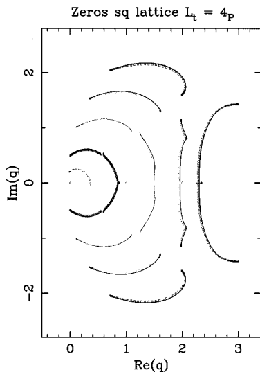
Fig. 7. Partition-function zeros in the complex q plane for the 4_p \times 40_F square-lattice strip for several values of the temperature-like parameter v : -1 ( \square ), -0.75 ( \circ ), -0.50 ( \triangle ), -0.25 ( \diamond ), and -0.10 ( \oplus ). The loci \mathcal{B} for the 4_p \times \infty_F strip for these values of v are also shown.
