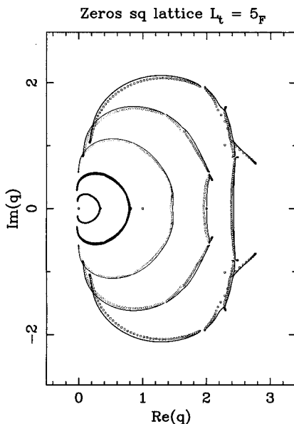
Fig. 4. Partition-function zeros in the complex q plane for the 5_F \times 40_F square-lattice strip for several values of the temperature-like parameter v : -1 ( \square ), -0.75 ( \circ ), -0.50 ( \triangle ), -0.25 ( \diamond ), and -0.10 ( \oplus ). The loci \mathcal{B} for the 5_F \times \infty_F strip for these values of v are also shown.
