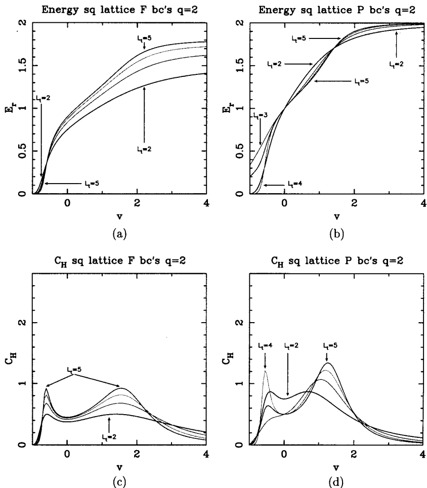
Fig. 13. Reduced internal energy E_r = -E/J and specific heat C_H as functions of the temperature-like parameter v for the q=2 Potts model on square-lattice strips of size (L_t)_F \times \infty_F and (L_t)_P \times \infty_P with 2 \leq L_t \leq 5 . The plot includes both the ferromagnetic and antiferromagnetic Potts models, for which the temperature ranges are 0 \leq v \leq \infty and -1 \leq v \leq 0 , respectively.
