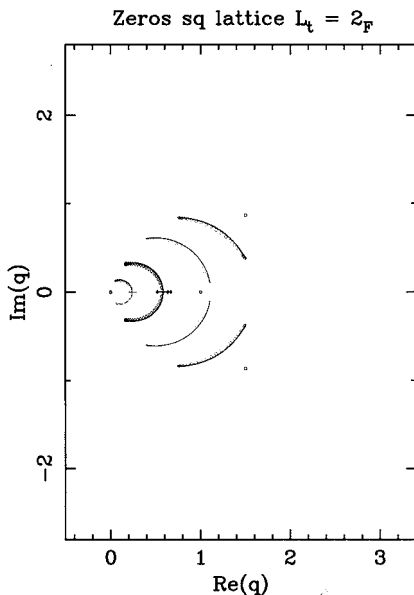
Fig. 1. Partition-function zeros in the complex q plane for the 2_F \times 20_F square-lattice strip and resultant accumulation set \mathcal{B} for the 2_F \times \infty_F strip (singular locus for the free energy) for several values of the temperature-like parameter v : -1 ( \square ), -0.75 ( \circ ), -0.50 ( \triangle ), -0.25 ( \diamond ), and -0.10 ( \oplus ), where the symbols correspond to the zeros calculated for the finite strip. The zero at q=0 is present for all v .
