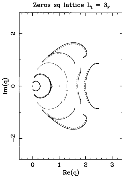
Fig. 2. Partition-function zeros in the complex q plane for the 3_F \times 30_F square-lattice strip for several values of the temperature-like parameter v : -1 ( \square ), -0.75 ( \circ ), -0.50 ( \triangle ), -0.25 ( \diamond ), and -0.10 ( \oplus ). The loci \mathcal{B} for the 3_F \times \infty_F strip for these values of v are also shown.
