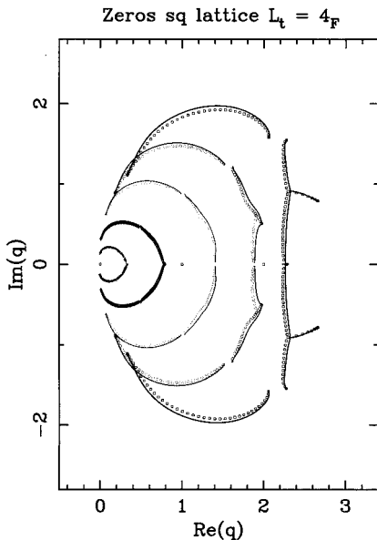
Fig. 3. Partition-function zeros in the complex q plane for the for the 4_F \times 40_F strip for several values of the temperature-like parameter v : -1 ( \square ), -0.75 ( \circ ), -0.50 ( \triangle ), -0.25 ( \diamond ), and -0.10 ( \oplus ). The loci \mathcal{B} for the 4_F \times \infty_F strip for these values of v are also shown.
