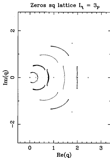
Fig. 6. Partition-function zeros in the complex q plane for the 3_p \times 30_F square-lattice strip for several values of the temperature-like parameter v : -1 ( \square ), -0.75 ( \circ ), -0.50 ( \triangle ), -0.25 ( \diamond ), and -0.10 ( \oplus ). The loci \mathcal{B} for the 3_p \times \infty_F strip for these values of v are also shown.
