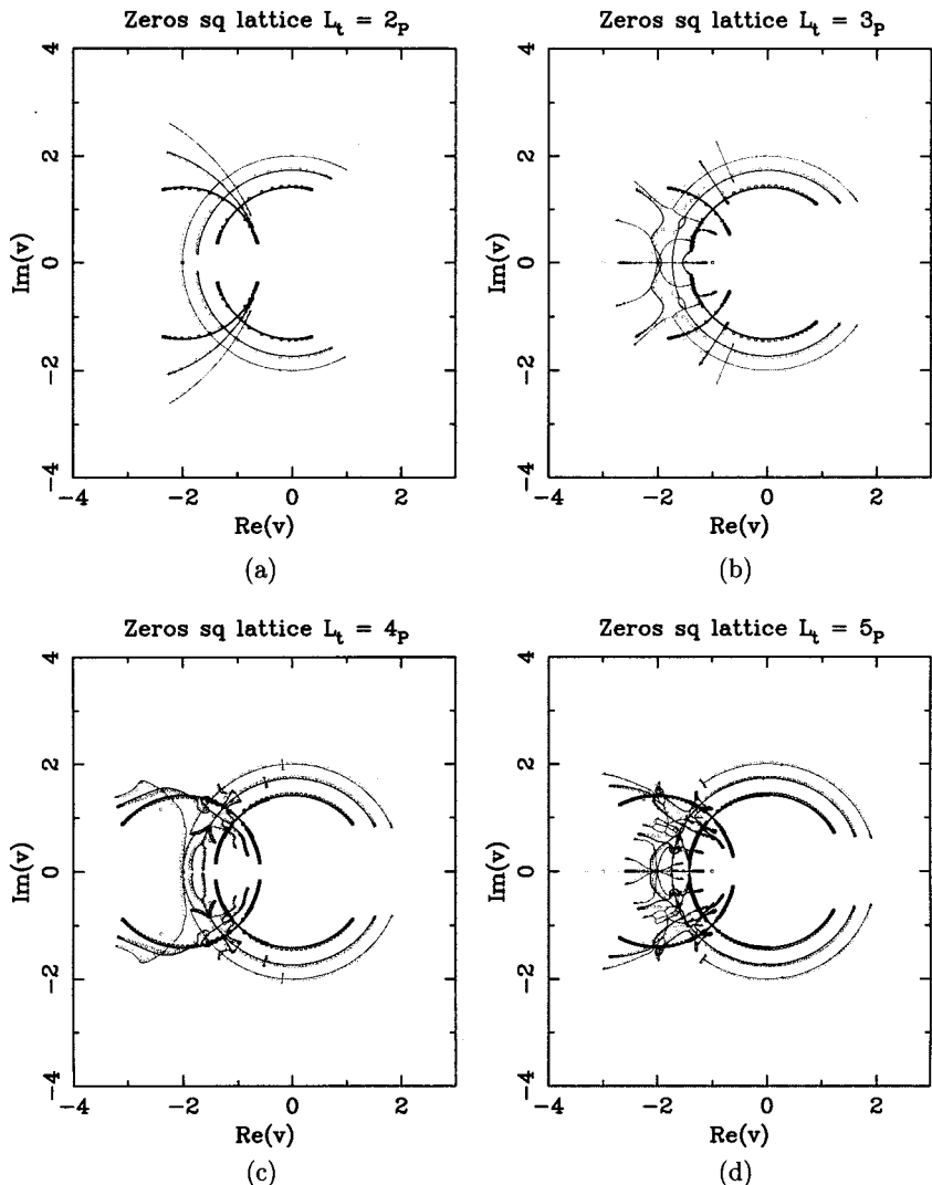
Fig. 10. Partition function zeros in the complex v plane for several square-lattice strips: (a) 2_p \times 20_F , (b) 3_p \times 30_F , (c) 4_p \times 40_F , and (d) 5_p \times 50_F . In each plot we show the zeros for several values of the parameter q : 2 ( \square , black), 3 ( \circ , red), and 4 ( \triangle , green) and the corresponding loci \mathcal{B} for these values of q . (Colors refer to the version of the paper online at cond-mat/0108144 .)
